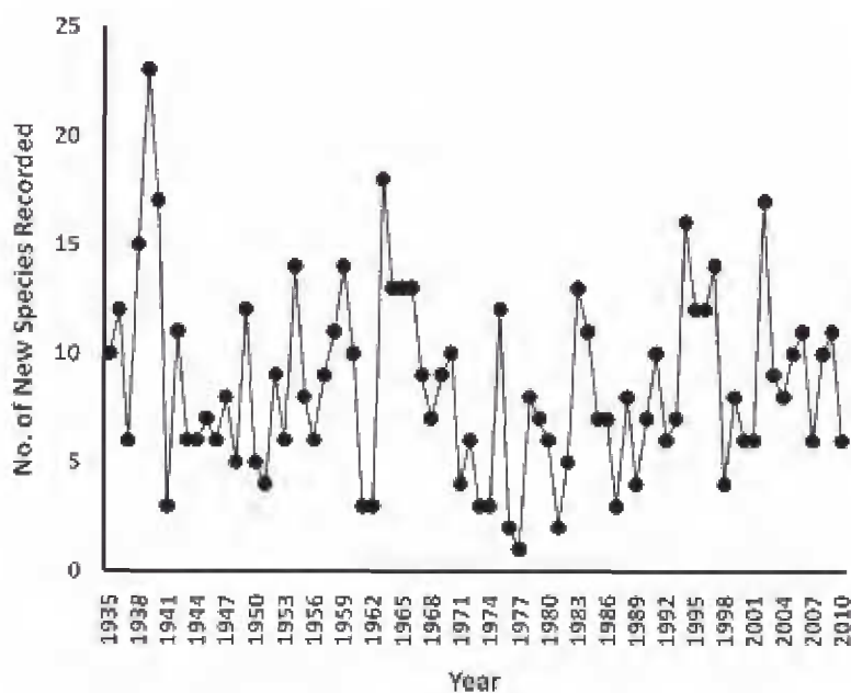
FIGURE 2. Total number of invertebrates detected in California 1935–2010.
